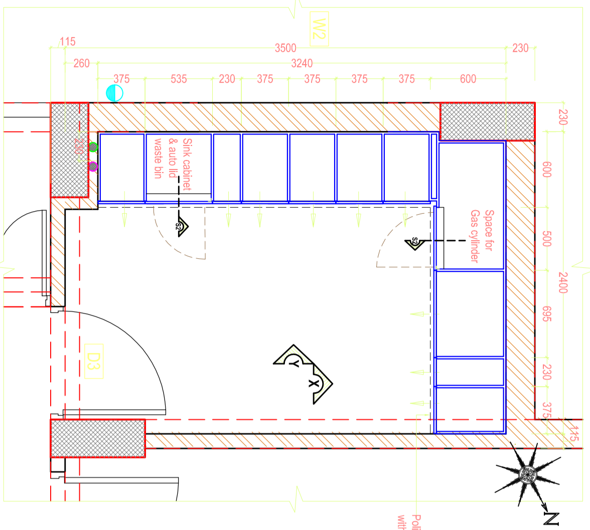
PLAN 'P2-P2'
