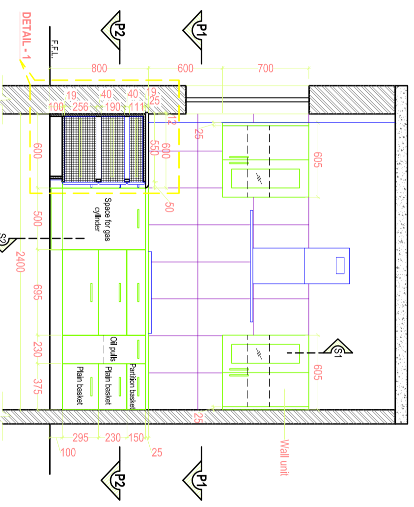
ELEVATION AT 'X'
