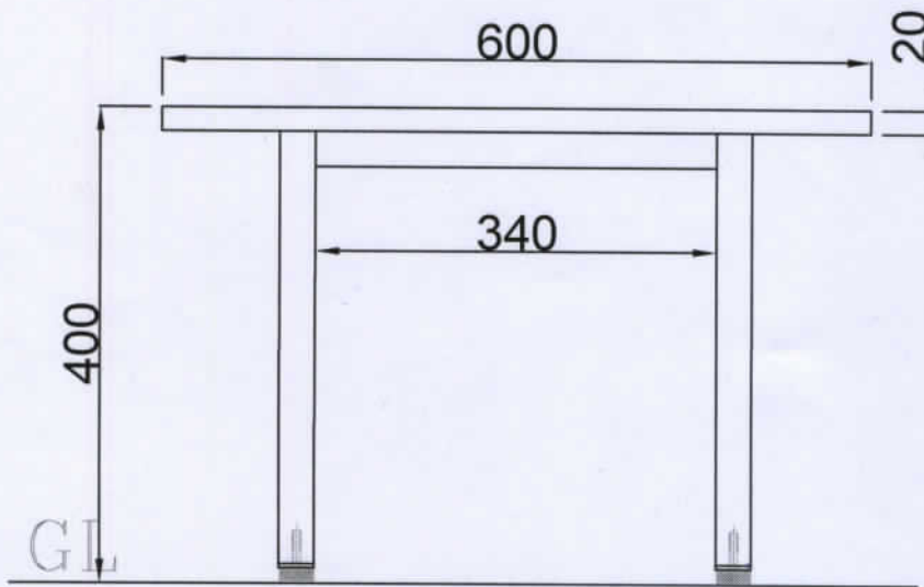
ELEVATION VIEW
