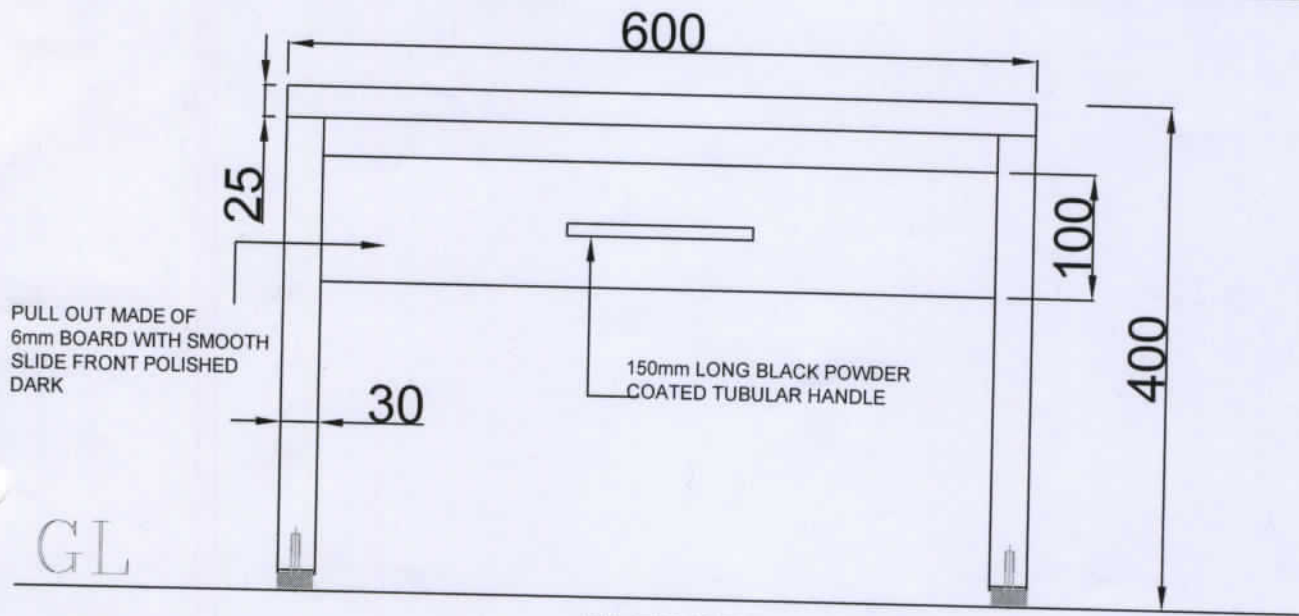
ELEVATION VIEW
