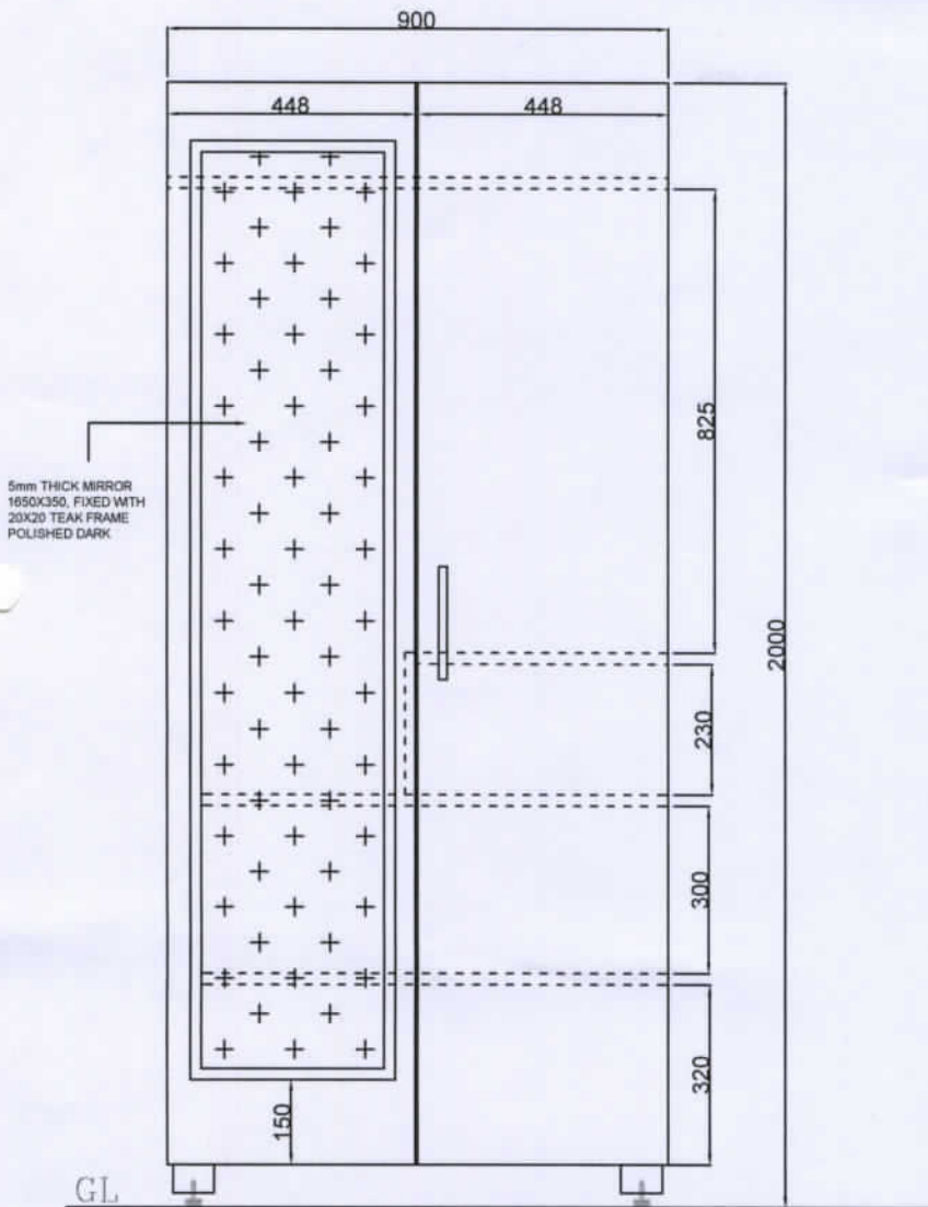
ELEVATION VIEW
