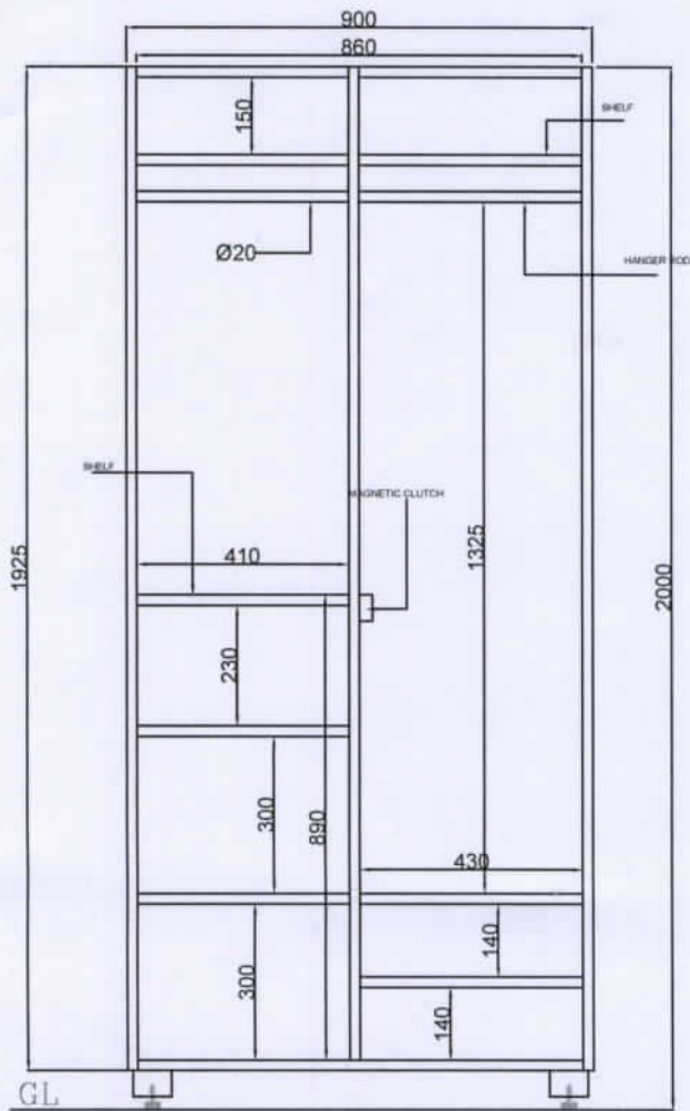
ELEVATION VIEW
