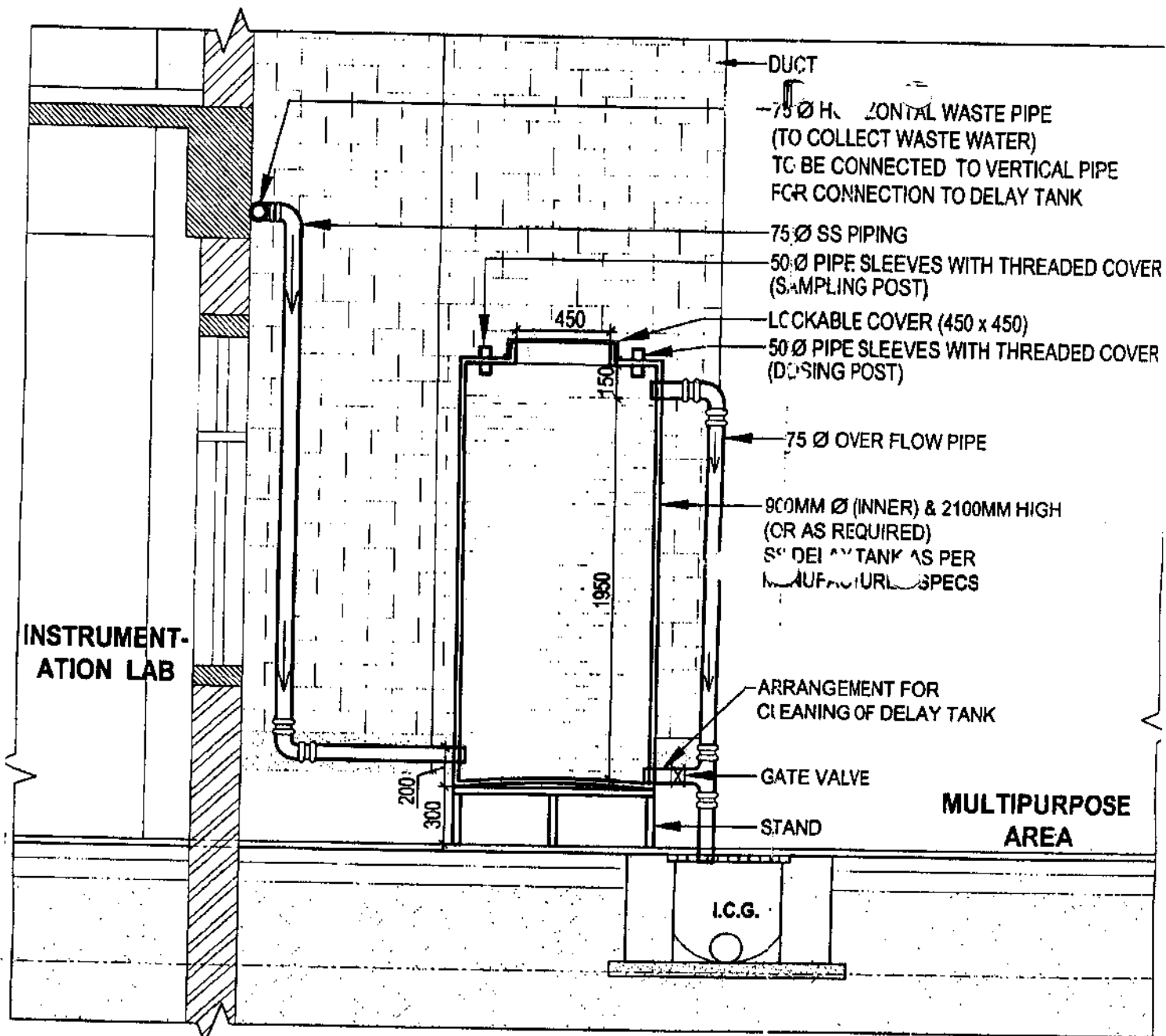
SECTION AT S-S
