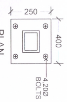
(SHOWING BOLTS ARRANGEMENTS TRUSS & COL.)
